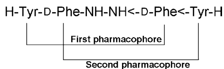
Figure 2. Opioid ligand with two overlapping pharmacophores. Relative affinities ( K_i ; nM) for \mu and \delta binding sites in guinea pig membranes: 31 \pm 2 ( \mu ); 187 \pm 15 ( \delta ). See Ref. 8.
