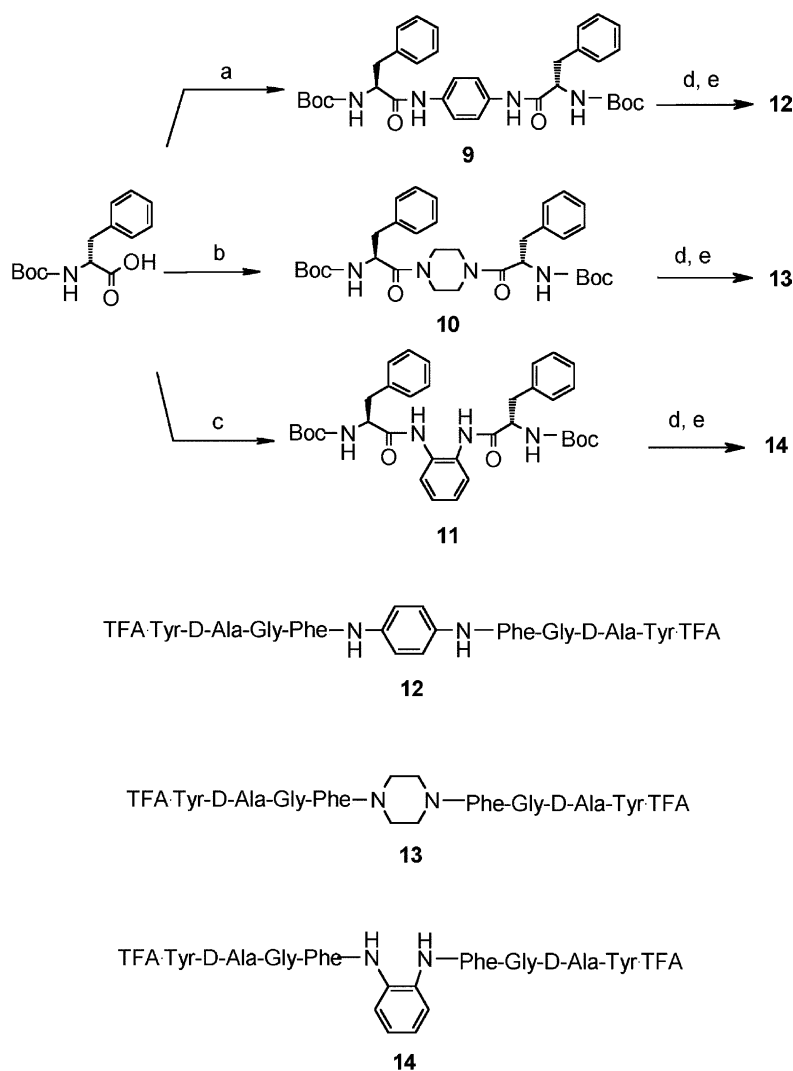
Scheme 3. Reagents and conditions: (a) Boc-L-Phe-OH (2.1 equiv), EDC (2.1 equiv), HOBT-H 2 O (2.1 equiv), TEA (3.2 equiv), 1,4-phenylenediamine·2HCl (1 equiv), DMF (20 mL), 30 min in 0 °C, then rt for 6 h; (b) Boc-L-Phe-OH (2.1 equiv), EDC (2.1 equiv), HOBT-H 2 O (2.1 equiv), TEA (2.2 equiv), piperazine·HCl (1 equiv), DMF (20 mL), 30 min 0 °C, then 6 h in rt; (c) Boc-L-Phe-OH (2.1 equiv), EDC (2.1 equiv), HOBT-H 2 O (2.1 equiv), TEA (3.2 equiv), 1,2-phenylenediamine·2HCl (1 equiv), DMF (20 mL), 30 min in 0 °C, then rt for 6 h; (d) TFA 50% in DCM 30 min rt under N 2 atmosphere, then Boc-Tyr-D-Ala-Gly-OH (2.1 equiv), EDC (2.1 equiv), HOBT-H 2 O (2.1 equiv), TEA (3.2 equiv), DMF (20 mL), 30 min, 0 °C, then rt for 6 h; (e) TFA 50% in DCM, 30 min rt under N 2 atmosphere. (Overall yield 30–50%).
