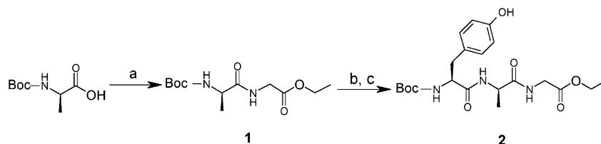
Scheme 1. Reagents and conditions: (a) H-Gly-OEt-HCl (1 equiv), i -BuOCOCi (1.1 equiv), TEA (1.1 equiv), DCM (20 mL), -15^{\circ}\text{C} for 15 min then rt for 12 h; (b) TFA 50%, DCM, rt for 30 min under N 2 atmosphere; (c) N^{\alpha} -Boc-Tyr-OH (1.1 equiv), i -BuOCOCi (1.1), TEA (1.1 equiv), DCM (20 mL), -15^{\circ}\text{C} for 15 min then rt for 12 h. (Overall yield 85%).
