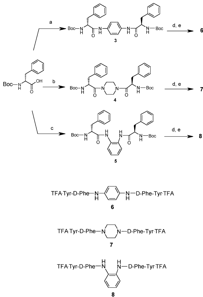
Scheme 2. Reagents and conditions: (a) Boc-D-Phe-OH (2.1 equiv), EDC (2.1), HOBT·H 2 O (2.1 equiv), TEA (3.2 equiv), 1,4-phenylenediamine·2HCl (1 equiv), DMF (20 mL), 30 min in 0 °C, then rt for 6 h; (b) Boc-D-Phe-OH (2.1 equiv), EDC (2.1 equiv), HOBT·H 2 O (2.1 equiv), TEA (2.2 equiv), piperazine·HCl (1 equiv), DMF (20 mL), 30 min in 0 °C, then rt for 6 h; (c) Boc-D-Phe-OH (2.1 equiv), EDC (2.1 equiv), HOBT·H 2 O (2.1 equiv), TEA (3.2 equiv), 1,2-phenylenediamine·2HCl (1 equiv), DMF (20 mL), 30 min in 0 °C, then rt for 6 h; (d) TFA 50% in DCM 30 min in rt under N 2 atmosphere, then Boc-Tyr-OH (2.1 equiv), EDC (2.1 equiv), HOBT·H 2 O (2.1 equiv), TEA (3.2 equiv), DMF (20 mL), 30 min in 0 °C, then rt for 6 h; (e) TFA 50% in DCM, 30 min rt under N 2 atmosphere. (Overall yield 30–50%).
